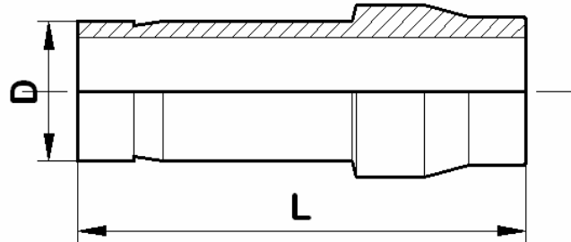
Port Connector
