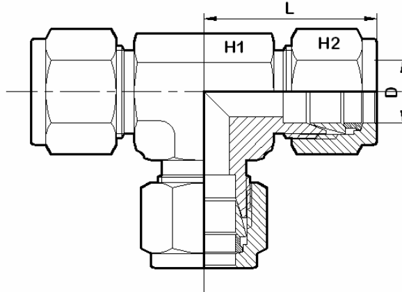
Union Tee
